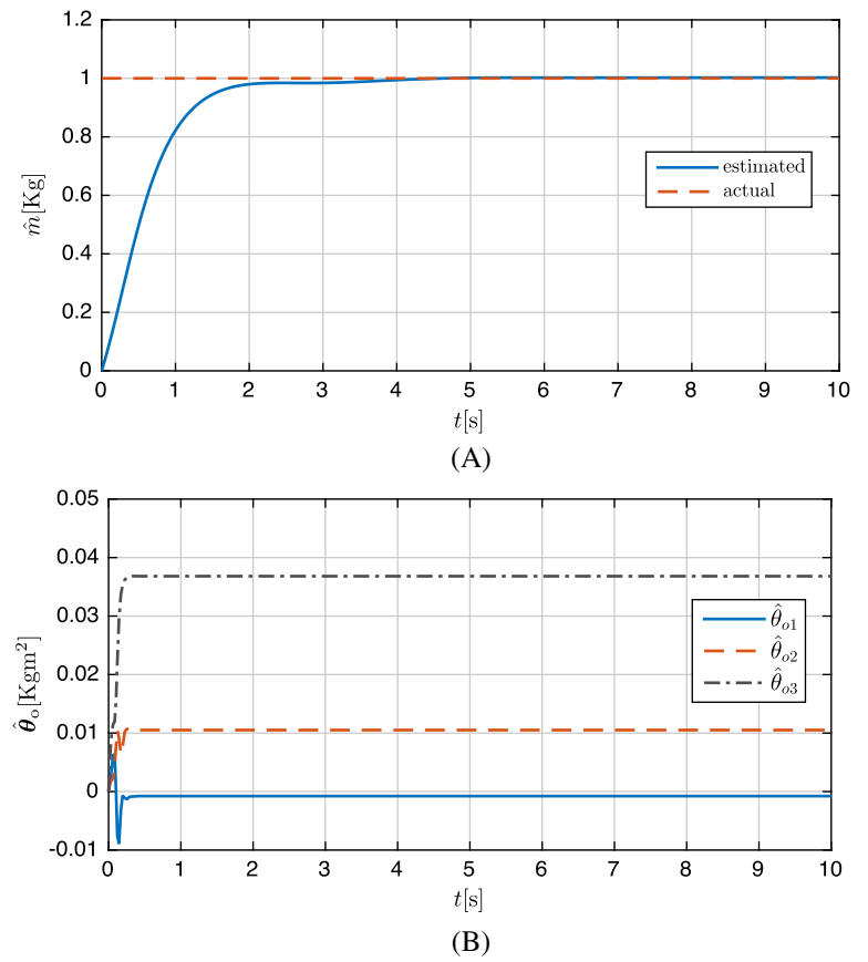
FIGURE 6 Trajectory of the estimated parameters: (A) mass and (B) inertia parameters [Colour figure can be viewed at wileyonlinelibrary.com ]
