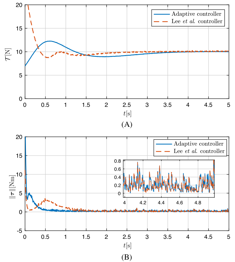
FIGURE 7 Control inputs: (A) total thrust \mathcal{T} and (B) torque \|\tau\| [Colour figure can be viewed at wileyonlinelibrary.com ]
